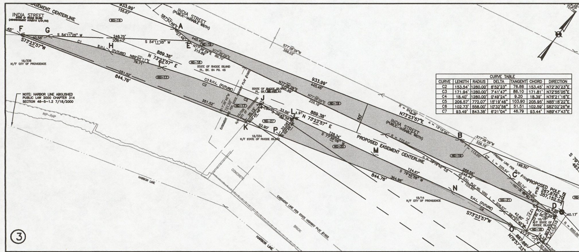
NOTE: Shaded area (A-B-C-D-E-A) indicates proposed transmission line easement. Total square footage = 13,828'± Shaded area (F-G-H-I-J-K-F) indicates proposed transmission line easement. Total square footage = 9,231'± Shaded area (L-M-N-O-P-L) indicates proposed transmission line easement. Total square footage = 7,000'±
