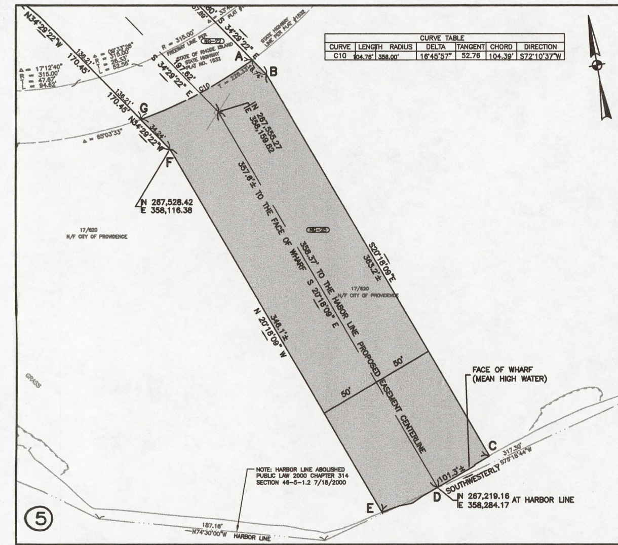
NOTE: Shaded area (A-B-C-D-E-F-G-A) indicates proposed transmission line easement. Total square footage = 37,981'±
