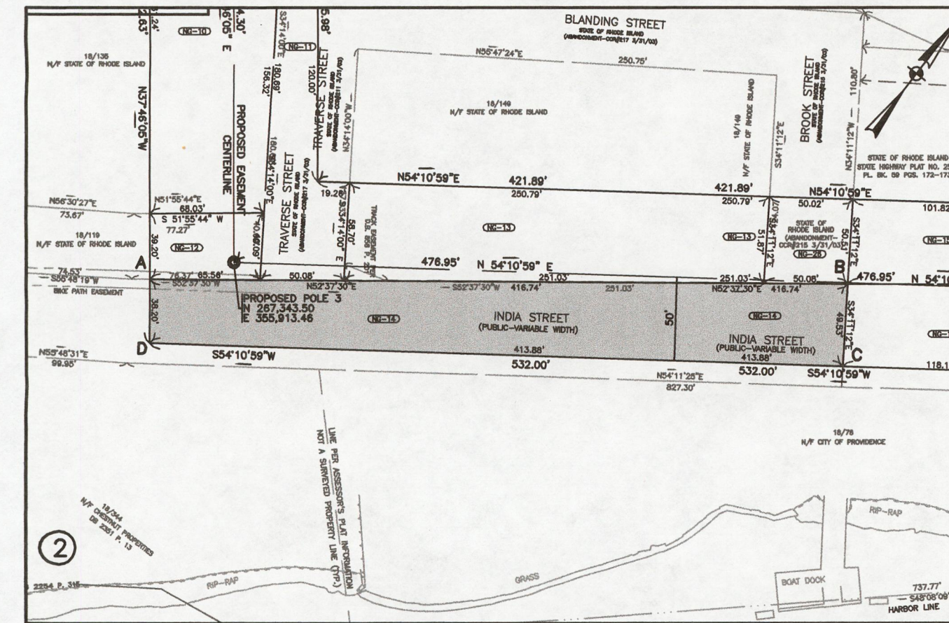
NOTE: Shaded area (A-B-C-D-A) indicates proposed transmission line easement. Total square footage = 18,207'±
