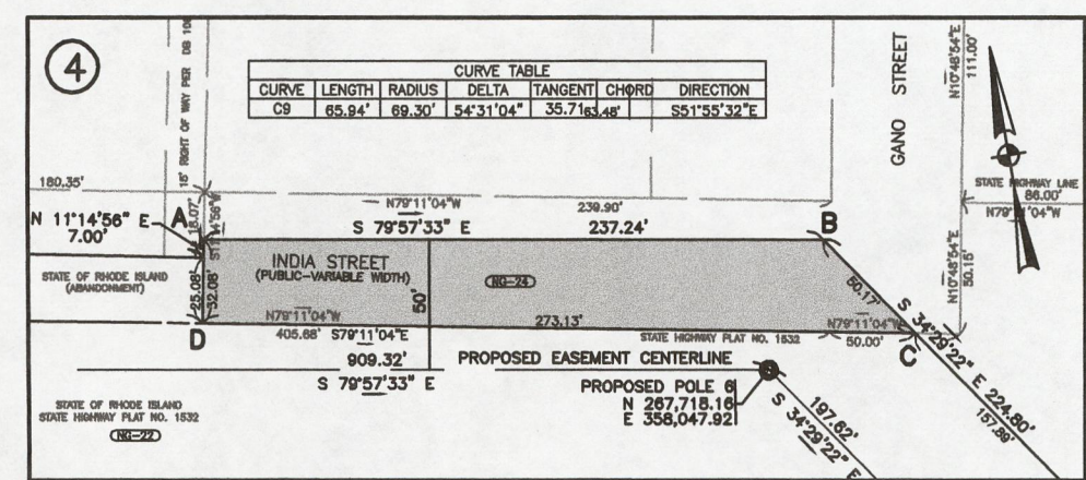
NOTE: Shaded area (A-B-C-D-A) indicates proposed transmission line easement. Total square footage = 8,623'±
