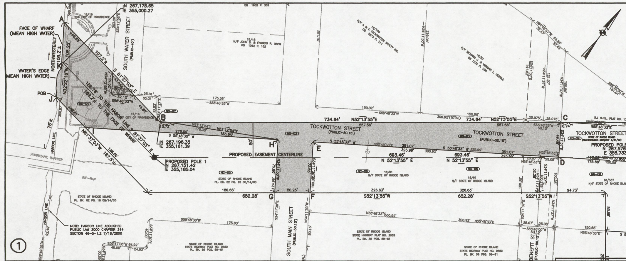
NOTE: Shaded area (A-B-C-D-E-F-G-H-I-J-K-A) indicates proposed transmission line easement. Total square footage = 32,970'±
