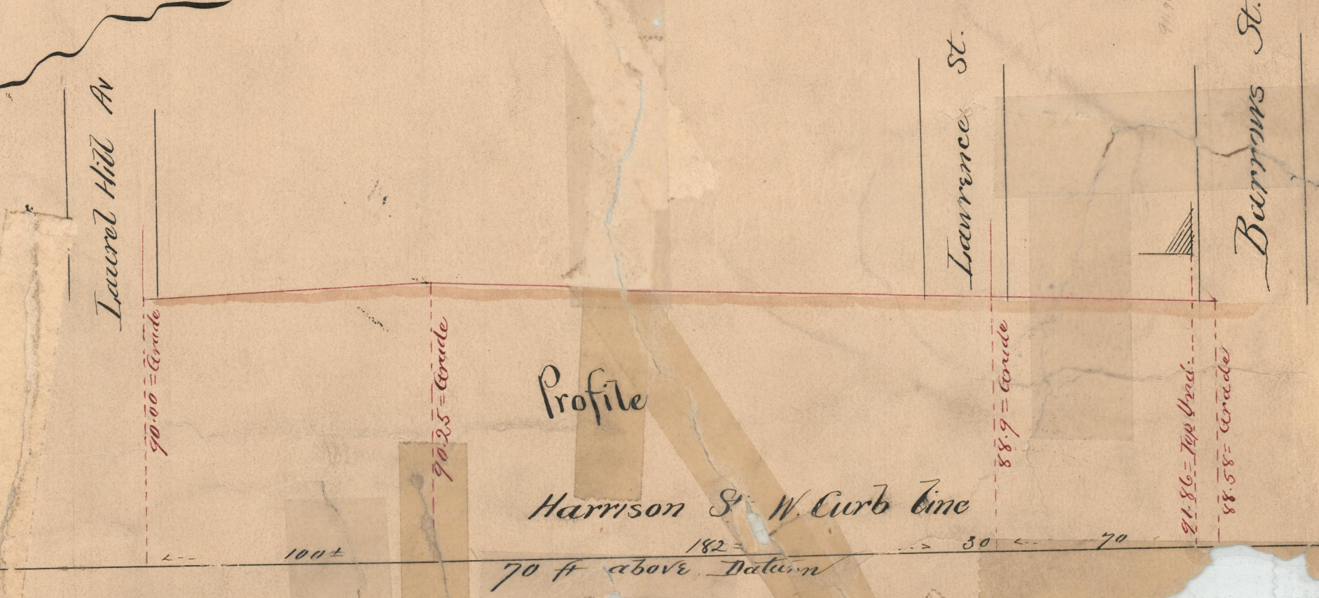
Profiles of REID and HARRISON STS JOHNSTON R.I. With Grades as defined by Highway Commissioners August 1894 R.S. Mowry Engineers
